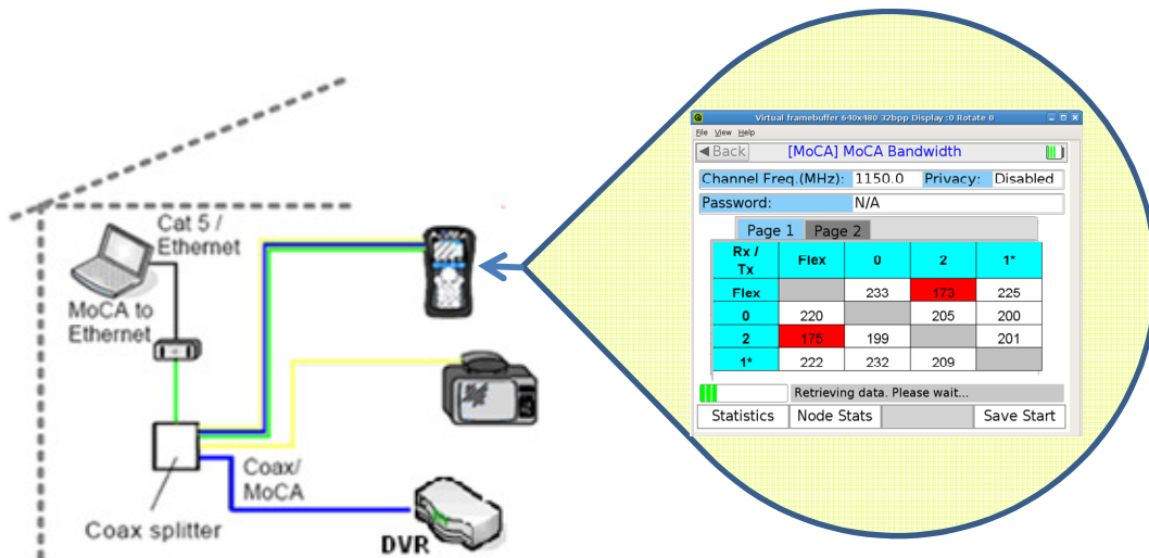
Figure 5. Inter-node throughput test
