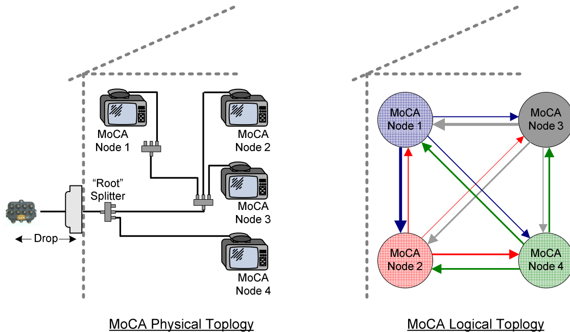
Figure 2. MoCA physical and logical topology
