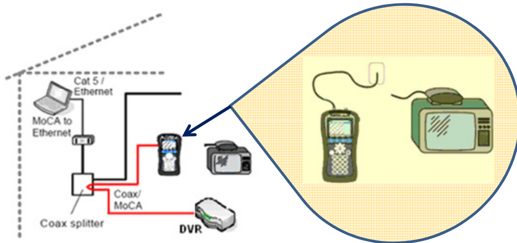
Figure 7. Coax integrity test
