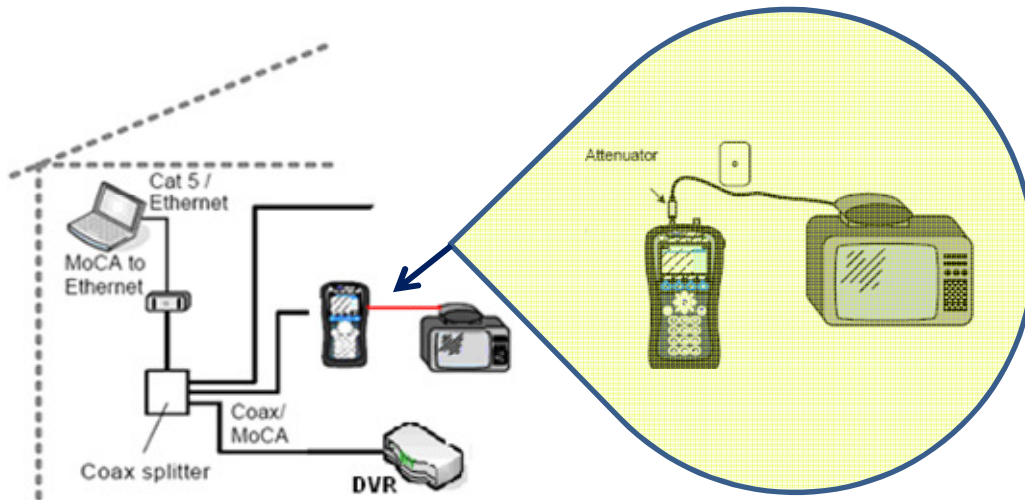
Figure 6. CPE output test
