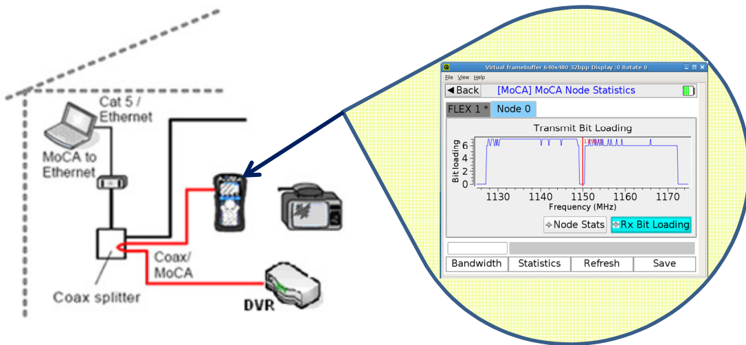
Figure 8. Interference test
