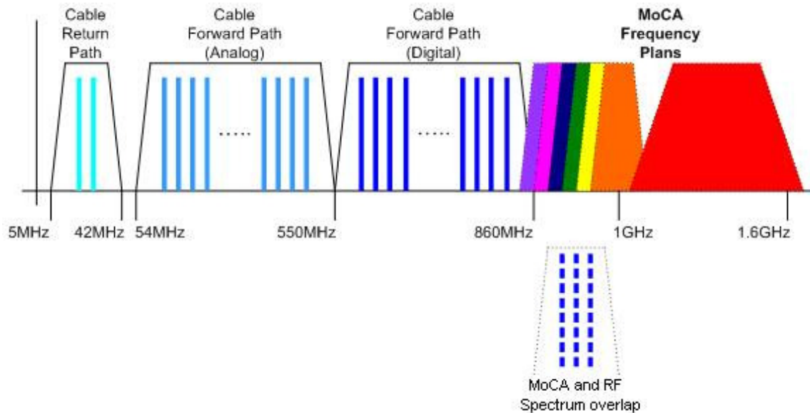
Figure 3. MoCA frequencies
